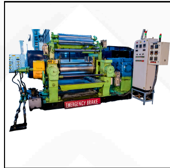
Mixing Mill with Stock Blender
